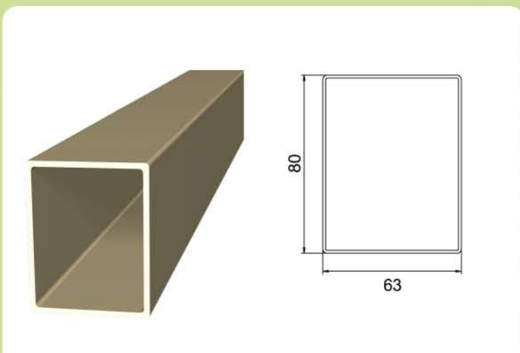
Vertical guide 80x63 mm
