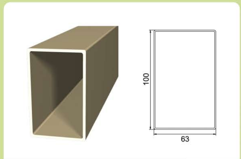
Vertical guide 100x63 mm
